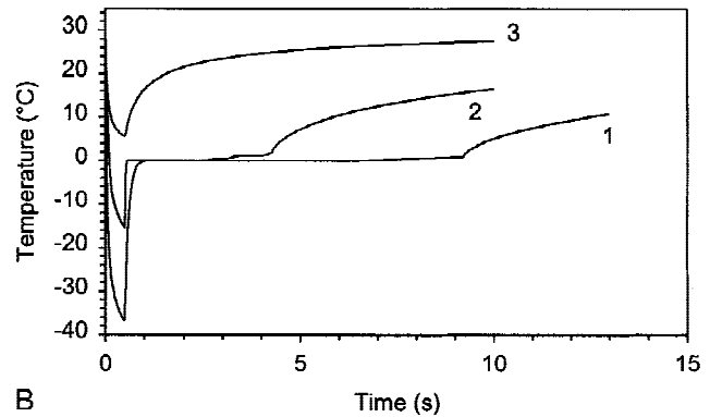
Fig. 6. A,B: Skin temperature at 100- \mu\text{m} depth versus time for hard-mode precooling. Initially, the skin surface temperature is kept constant for 100 ms (a) or 500 ms (b) at -50^\circ\text{C} (1), -26^\circ\text{C} (2), and 0.1^\circ\text{C} (3) by thermal contact with the CA. The cooling agent is then removed at the end of the precooling time.
